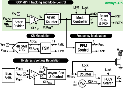
Fig. 3. Schematic of the MPPT and supporting control circuits. Shaded area indicates always-on blocks.
