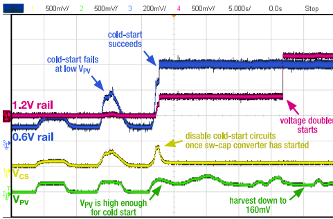
Fig. 5. PV cold-start showing 0.6V and 1.2V supply rails. Once the the 0.6V rail has booted, CS circuits are power-gated
