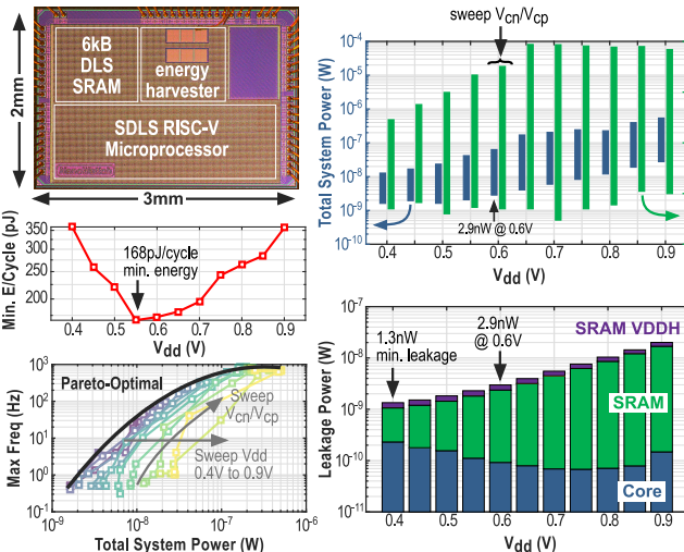
Fig. 8. NanoWatch die photo, measuring perf. scaling range vs. V_{DD} and V_{cn}/V_{cp} , min. E/cycle, pareto-optimal performance, and leakage breakdown.
