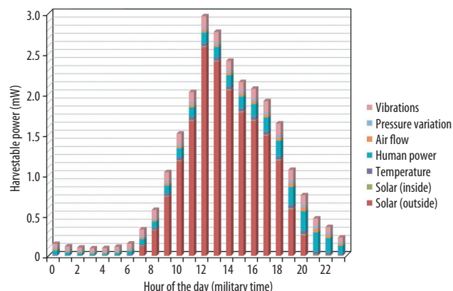
Figure 5. Results of correlating seven energy-harvesting sources with each source's availability over an average workday. Each segment represents the average amount of power that an individual could expect to harvest at any given time when all sources are being deployed. Nightly blackouts are a particular challenge and will require efficient energy storage mechanisms.
